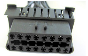
OBD2-FR-MB11
